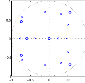
Fig. 3. ARMA 2 \times 2 model, with order n = 6 .
