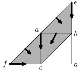
Figure 2.2: A complex \Delta along with a matching M on the family of faces outside the subcomplex \Delta_0 with maximal faces bc, bd, cd .
