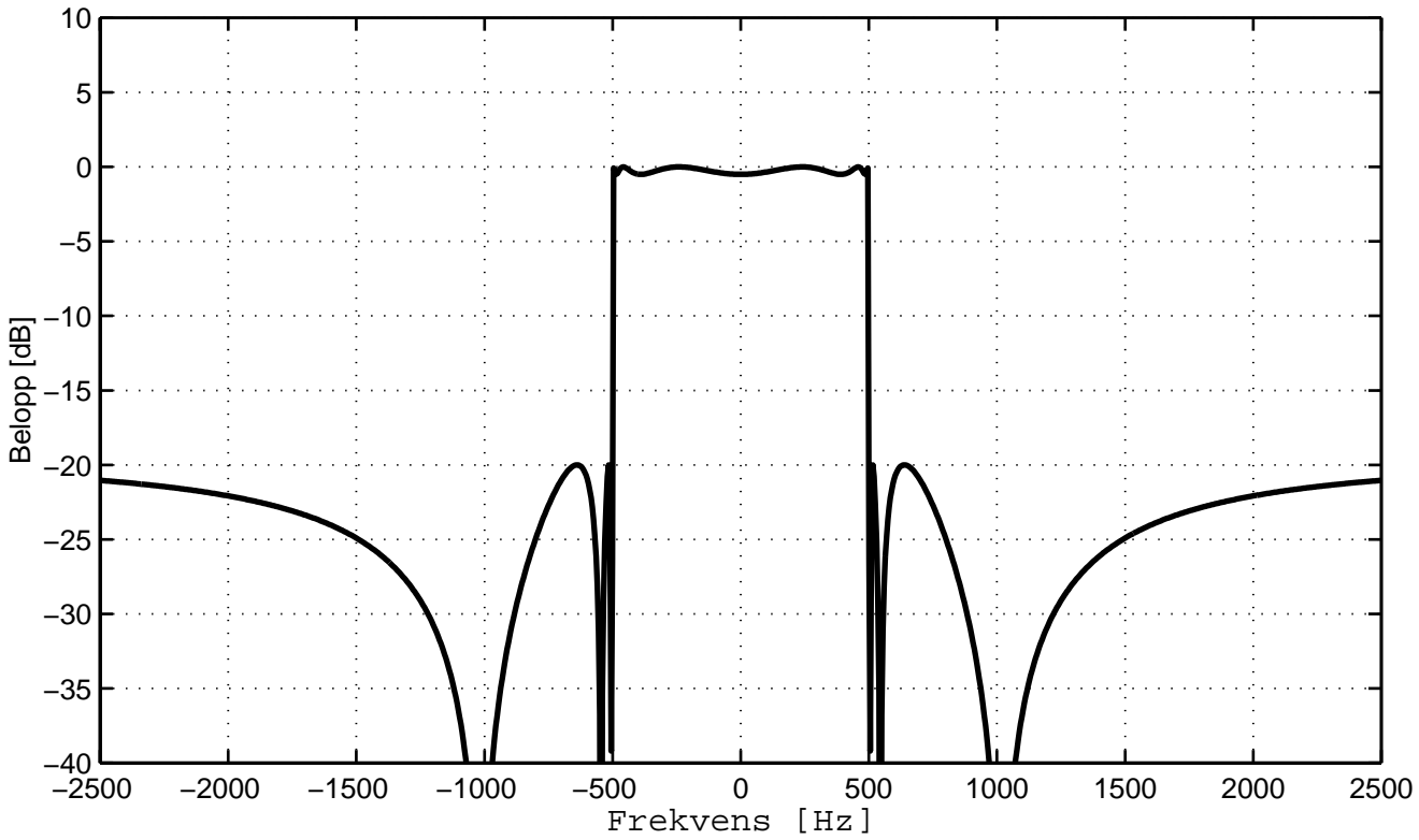
LP-filter
