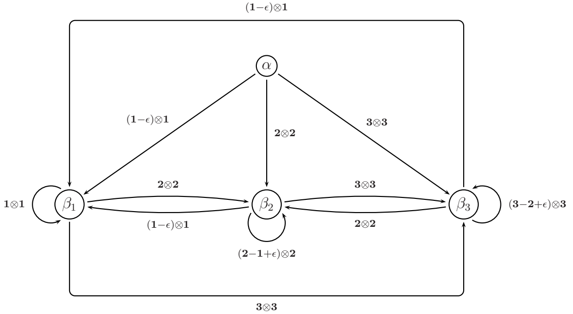
Figure 2: The automaton for M_\otimes when n = 3
