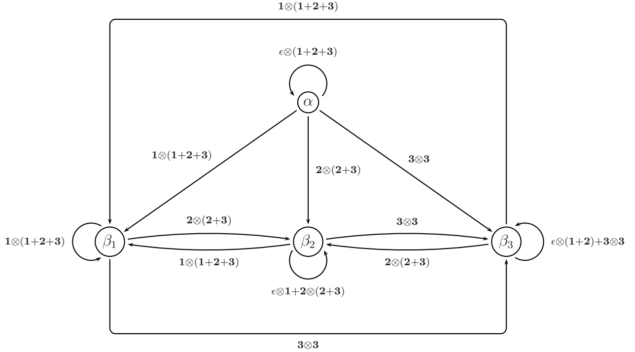
Figure 1: The automaton for Z_{\otimes} when n = 3
