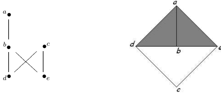
Fig. 1: A finite space and its associated simplicial complex.
