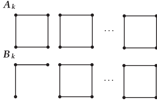
FIGURE 8. Graphs A_k and B_k .
