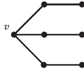
FIGURE 3. The graph W .
