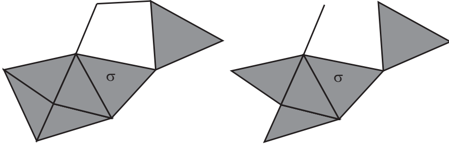
FIGURE 1. A 2-dimensional clique complex at the left and the star cluster of a simplex \sigma at the right.
