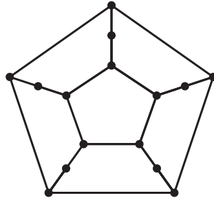
FIGURE 2. The graph described above for n = 5 .
