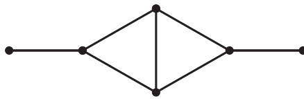
FIGURE 7. A claw-free graph whose independence complex is not a matching complex.
