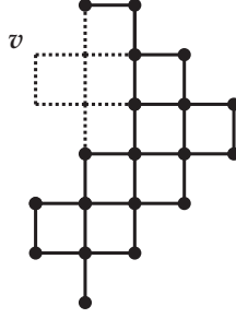
FIGURE 4. The graph \tilde{G}(7,6,3) . The complex st(v) \cap SC(N(v)) is the independence complex of the subgraph \tilde{G}(7,6,6) induced by the round vertices.
