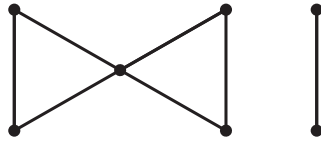
FIGURE 6. A claw-free graph G such that \tilde{H}_k(I_G) \neq 0 only for k = 1 and k = 2 .
