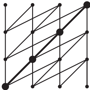
FIGURE 5. A poset with a chain that intersects all the maximal chains.
