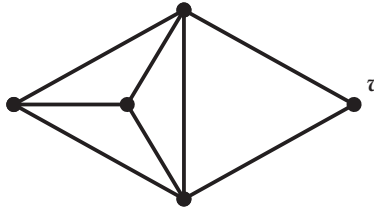
FIGURE 9. The graph G in Example 6.4.
