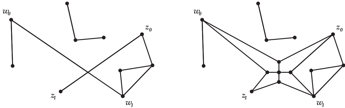
FIGURE 10. In the graph at the left two edges intersect. At the right, a suspension of the graph embedded in the plane.
