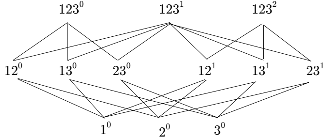
Figure 1. (B_3 \setminus \{\emptyset\}) * C_2
