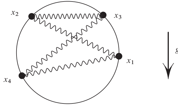
FIGURE 1.2. A mechanical interpretation of (1.3) with the coupling \beta(x_{i-1}, x_i, x_{i+1}) = \sin(x_{j-1} - 2x_j + x_{j+1}) .
