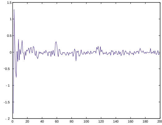
FIG. 4. Cepstrum of voice speech signal.
