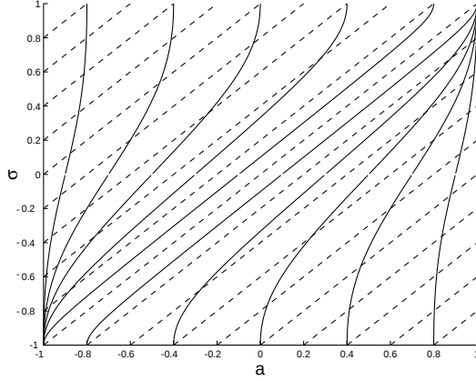
FIG. 5. Cepstral (dotted line) and covariance (solid line) matching foliations of \mathcal{P}_1 .
