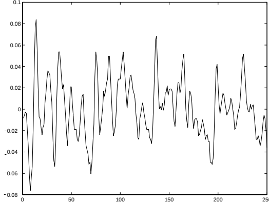
FIG. 2. A frame of speech for the voiced nasal phoneme [ng].
